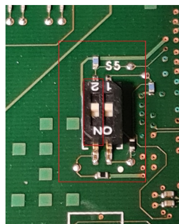
Figure 2. Switch S5_2 after change (OFF)
