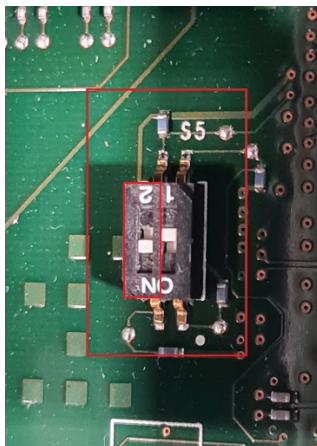
Figure 1. Switch S5_2 before change (ON)
