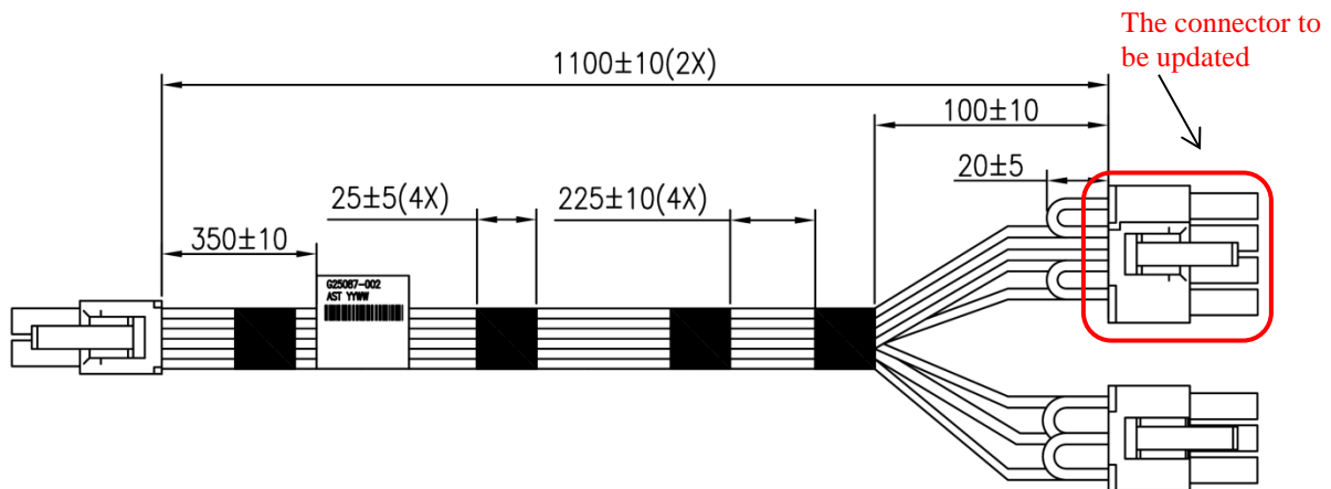
Figure-1 GPGPU Power Cable
