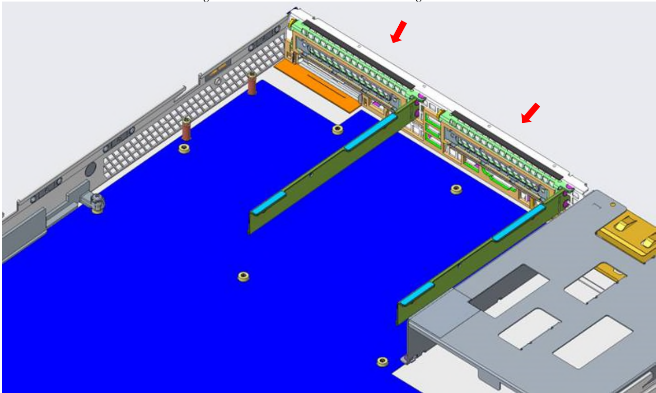
Figure 2. 1U Riser bracket with the new gasket.
