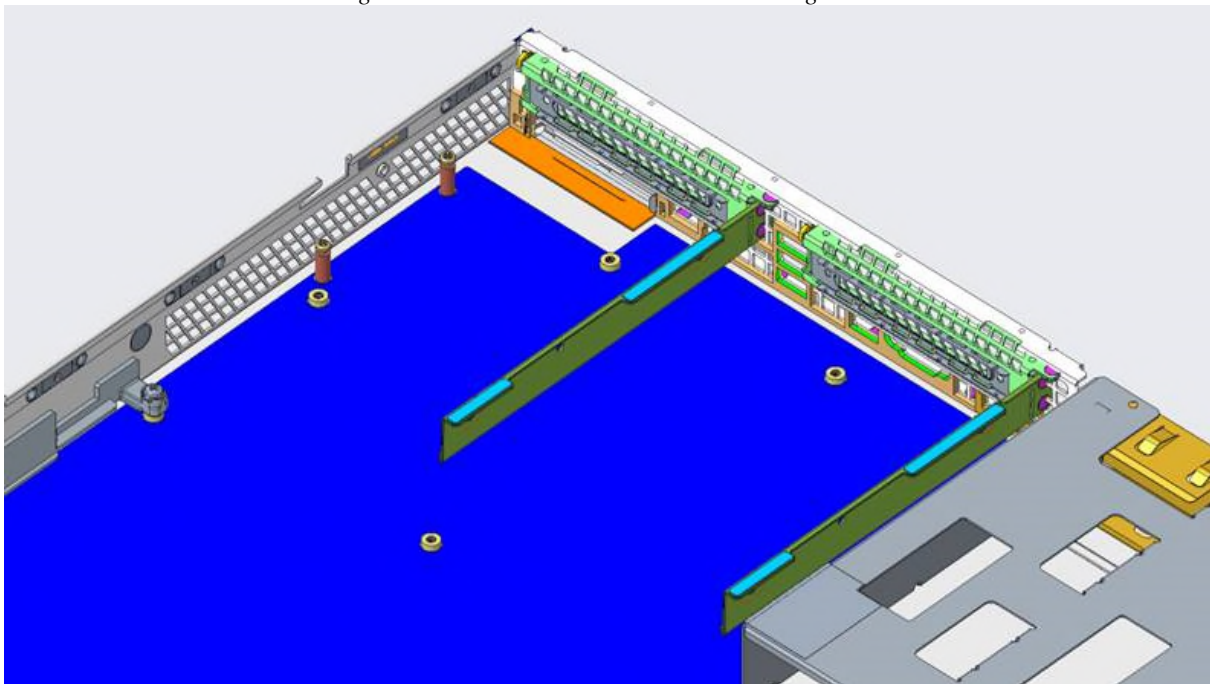
Figure 1. 1U Riser bracket without the new gasket.
