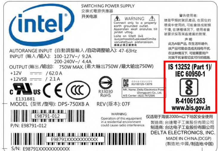
Image 2. Power supply label after change
