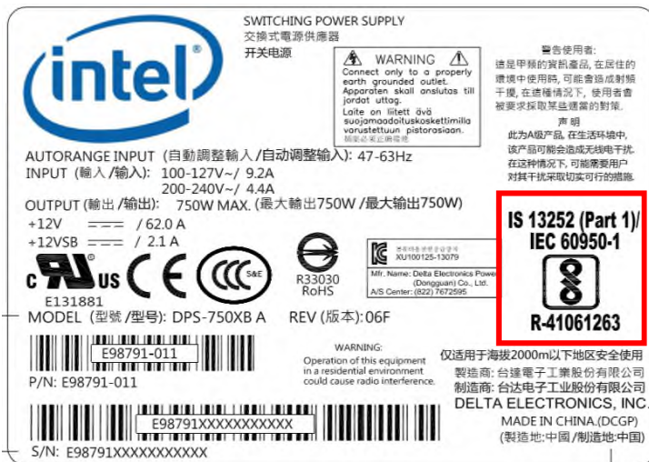
Image 1. Power supply label before change
