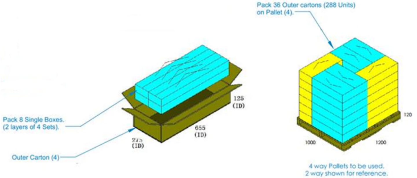
Image 4. New bulk carton box and pallet design
