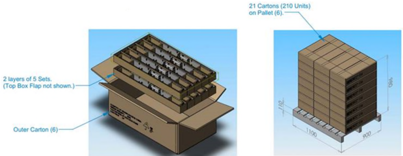
Image 3. Previous bulk carton box and pallet design
