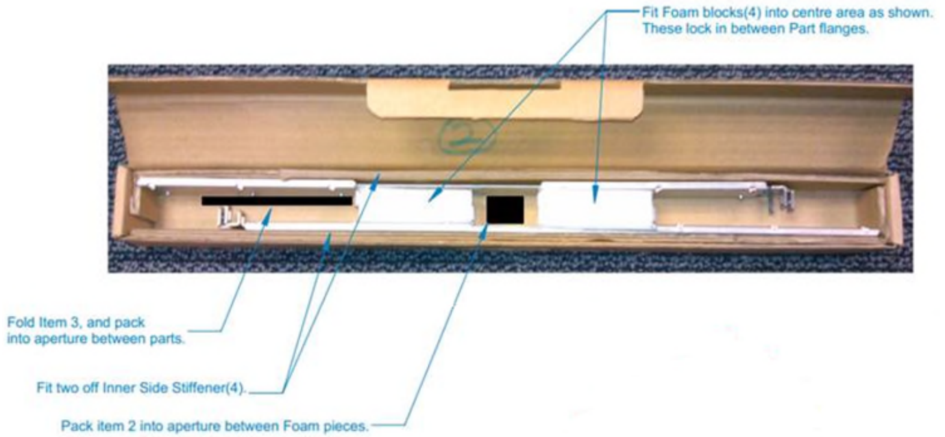
Image 2. Single carton box – New foam design
