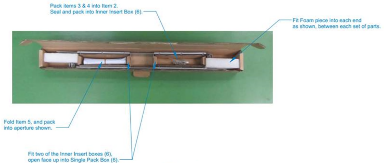
Image 1. Single carton box previous foam design
