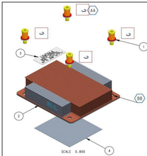
Figure 1. heatsink before change
