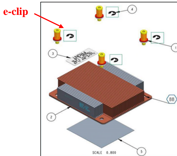
Figure 2. heatsink with “e-clip”
