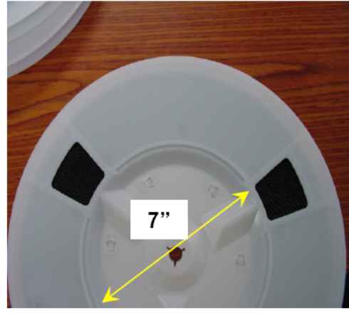
New Hub design, 550 units / reel
