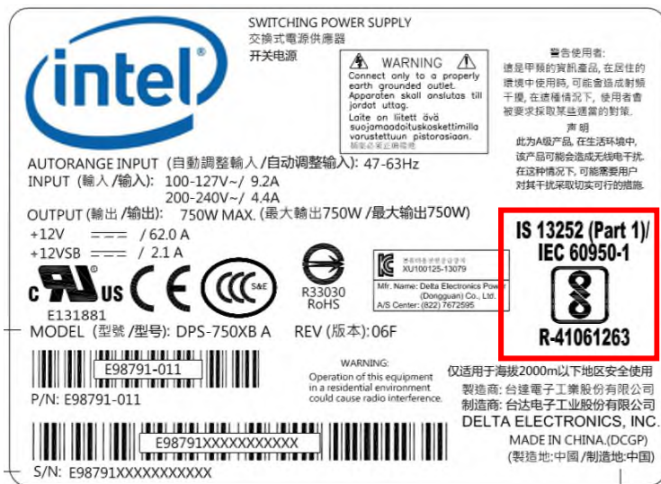
Image 1. Power supply label before change
