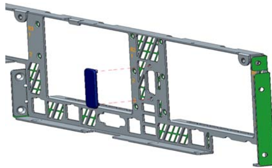
Image 1 “DB9 rear panel hole”
