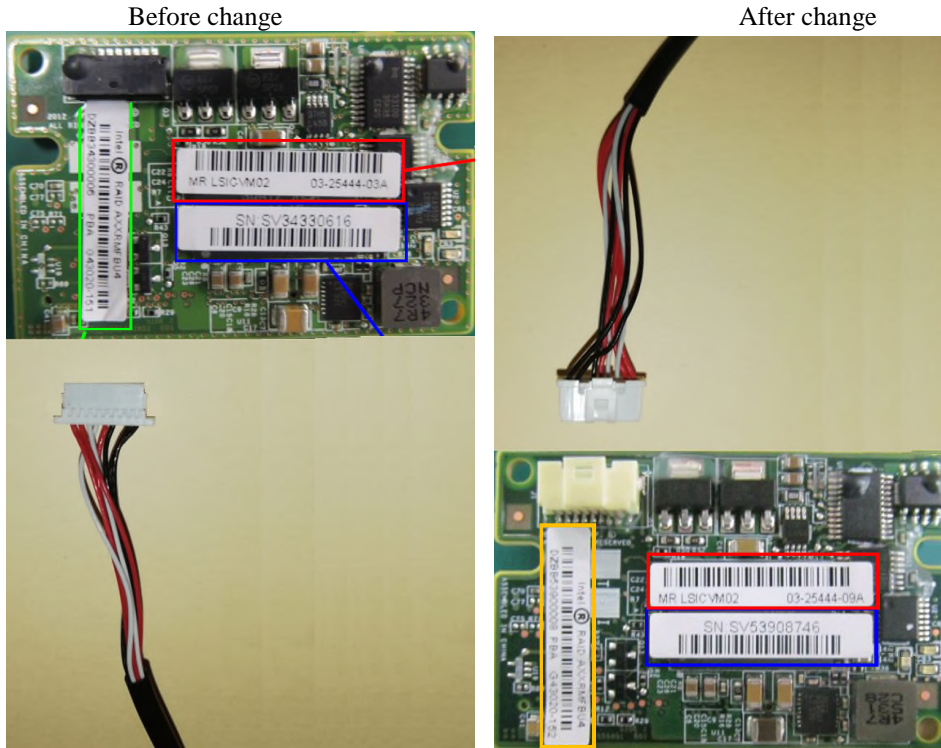
Figure1. Connector and cable change
