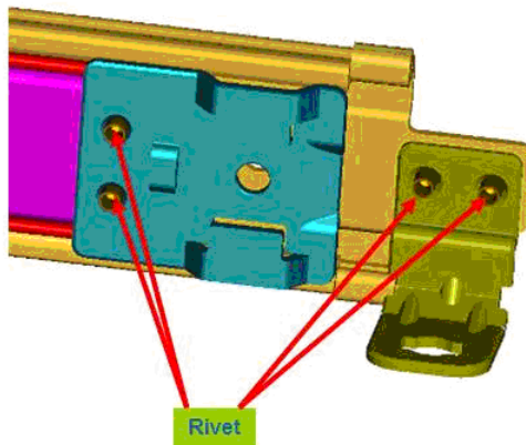
Current design-4 rivets per rail arm
