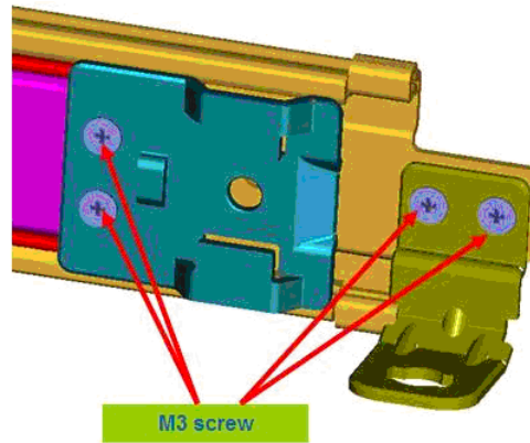
After change-4 screws per rail arm
