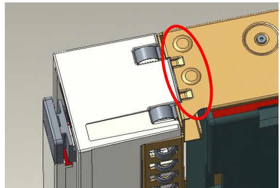
Figure 2: New shape with groove
