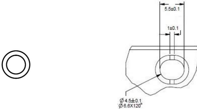
Figure-3: Node screw hole opening (Pre-Change)
