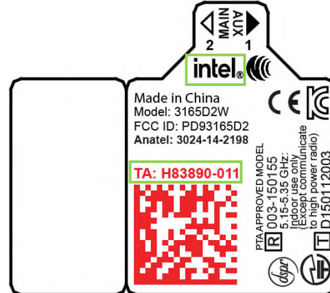
3165.D2WG Product Label - After
