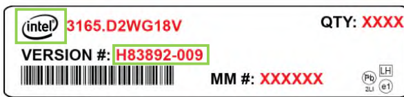
3165.D2WG18V Reel Label - Before
