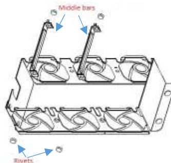
Fan cage with the changes
